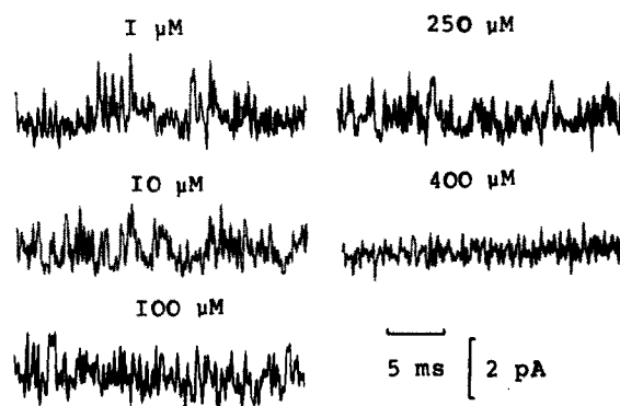
Fig.3. Fluctuations of the current through single cGMP-dependent channel at various 8BrGMP concentrations, range of milliseconds. Membrane voltage is -70 mV.
